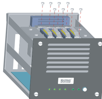
2) Push the drives into SATA connector completely, and secure the drives with screws.
